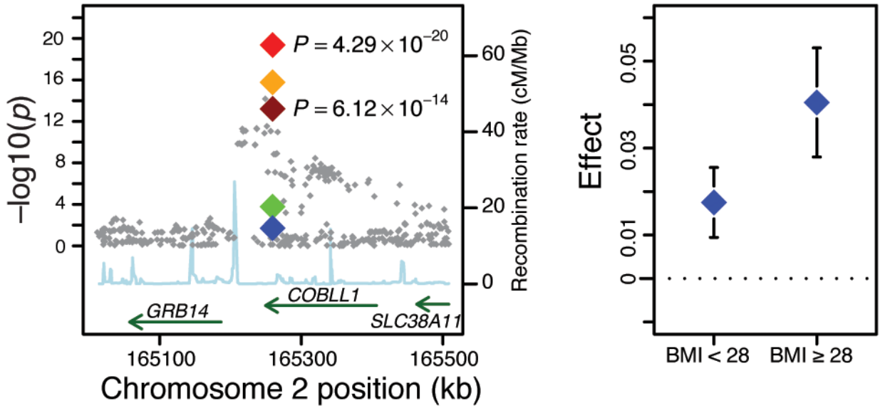
Figure 2. Regional plot of the COBLL1-GRB14 genomic locus. The left plot shows the discovery JMA P values in the background and for the SNP taken forward to the follow-up analyses (rs7607980), the P values of the discovery JMA (dark red) and the combined discovery and follow-up JMA (light red), main effects adjusting for BMI (orange), interaction with continuous BMI (green) and interaction with dichotomous BMI (blue). The right plot shows the beta estimates with 95% confidence interval of the increasing allele in the two BMI strata: BMI < 28 and BMI \geq 28 kg/m 2 . Effect = Beta estimates from regression models of ln(FI) adjusting for age, sex and other study-specific covariates.
